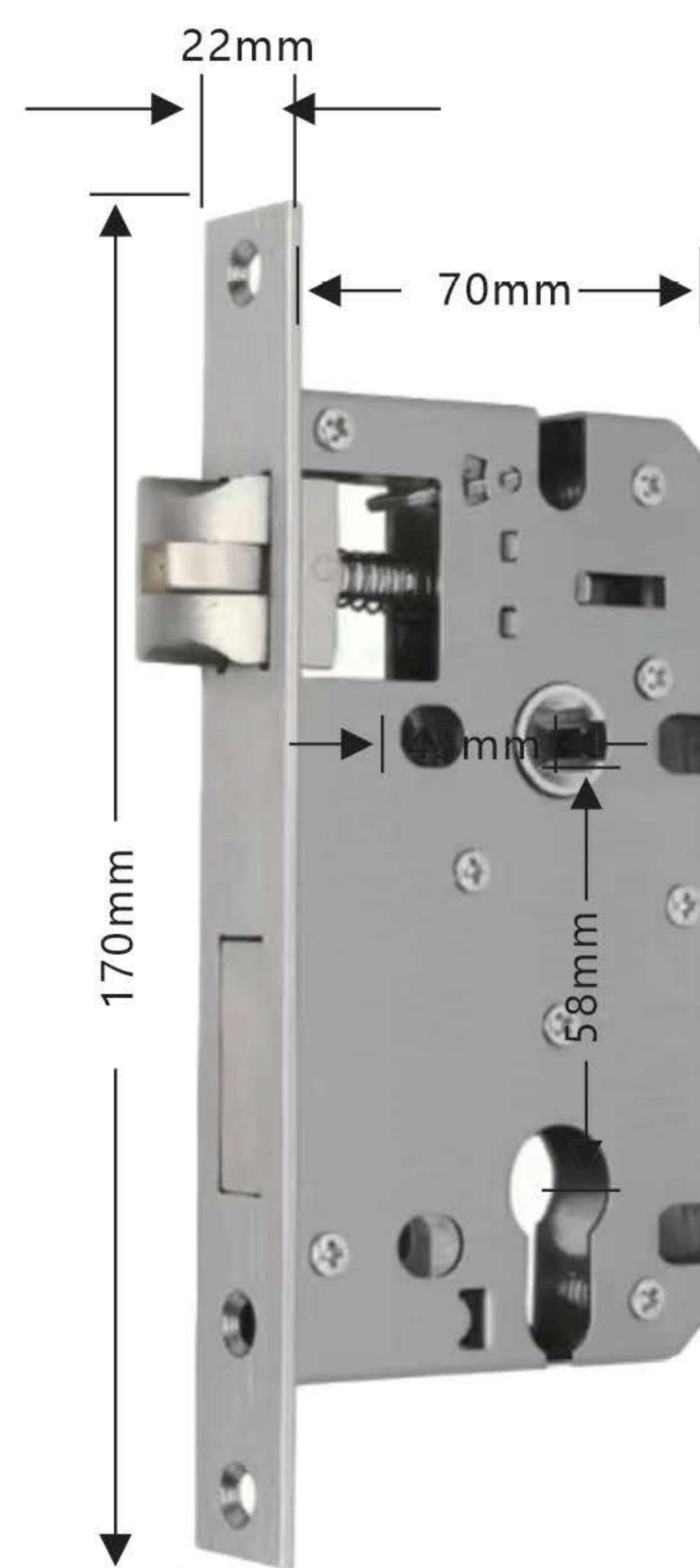
4558 lock body
