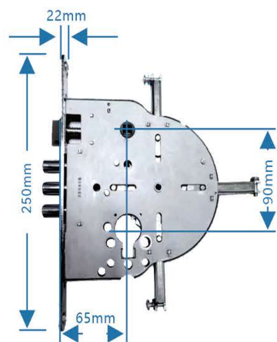
Israeli Lock Body
